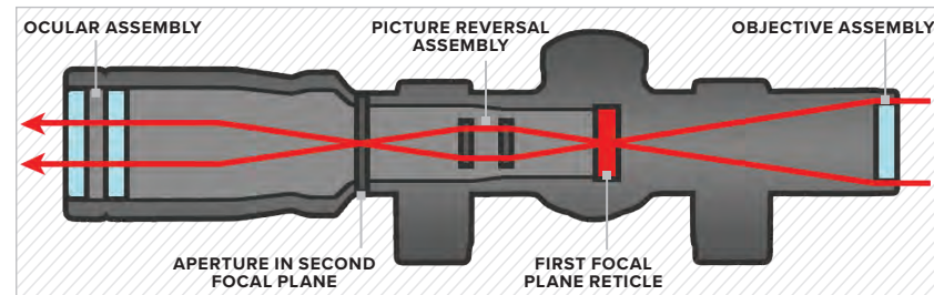
TRI-ILLUMINATED RETICLE SIGHTS
